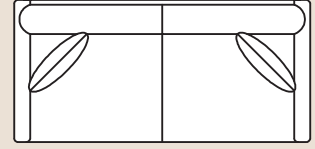
2275 Studio Sofa Overall: H 36 W 74 D 38 Seating: H 16 W 64 D 21 Seat Height: 20 Arm Height: 25 Pillows: 2 P23
