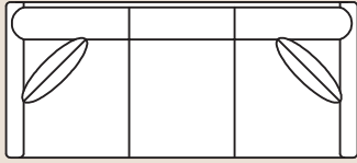
2200 Sofa Overall: H 36 W 80 D 38 Seating: H 16 W 72 D 21 Seat Height: 20 Arm Height: 25 Pillows: 2 P23
