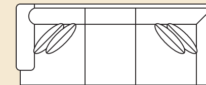
9262 LAF Corner Sofa 9263 RAF Corner Sofa Overall: H 39 W 99 D 40 Seating: H 18 W 74 D 24 Seat Height: 21 Arm Height: 24 Pillows: 4 P23
