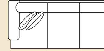
9252 LAF One Arm Sofa Overall: H 39 W 83 D 40 Seating: H 18 W 71 D 24 Seat Height: 21 Arm Height: 24 Pillows: 2 P23
