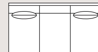
2484 Armless Sofa Overall: H 37 W 75 D 41 Seating: H 17 W 75 D 23 Seat Height: 20 Arm Height: N/A Pillows: 2 P21
