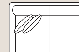
2372 LAF One Arm Loveseat 2373 RAF One Arm Loveseat Overall: H 37 W 59 D 43 Seating: H 18 W 54 D 23 Seat Height: 19 Arm Height: 25 Pillows: 2 P22
